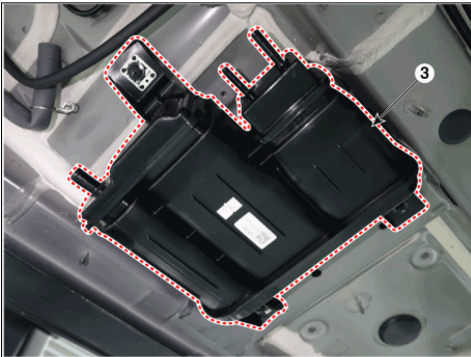
5. GPF (Gasoline Particulate Filter)
